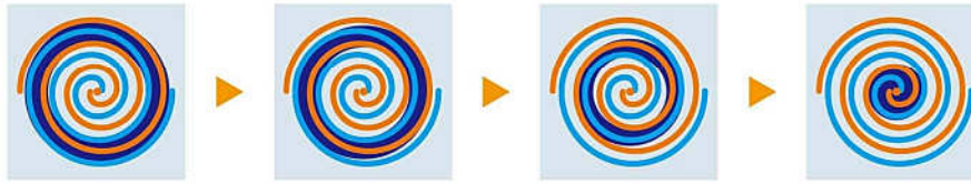
— Orbiting Scroll Rotor 動盤 — Fixed Scroll Stator 靜盤 — Compression Room 壓縮室
